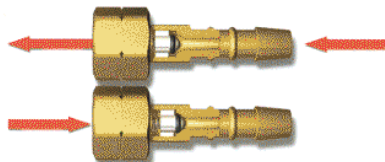
Poistka BV 12 kyslík Poistka BV 12 acetylén Non-return valve BV 12 oxygen Non-return valve BV 12 acetylene
