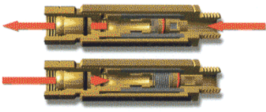
Suchá predloha SP 20 kyslík Suchá predloha SP 20 acetylén Flashback arrestor SP 20 oxygen Flashback arrestor SP 20 acetylene
